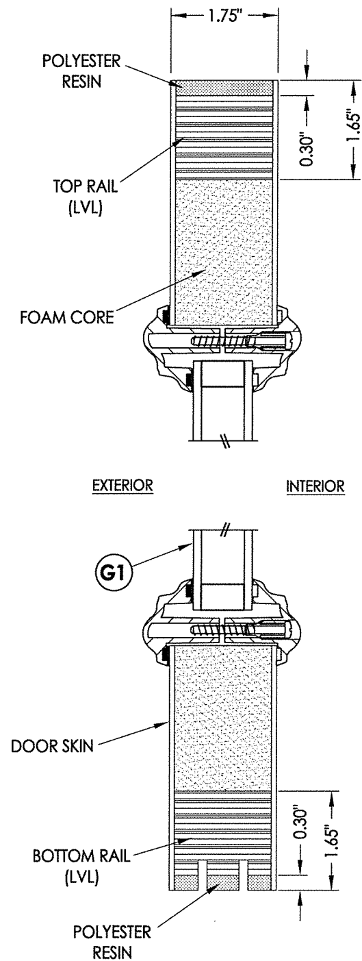
2 VERTICAL CROSS SECTION
