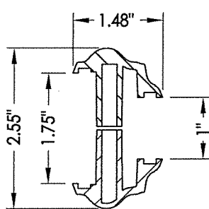
G1 GLAZING DETAIL
