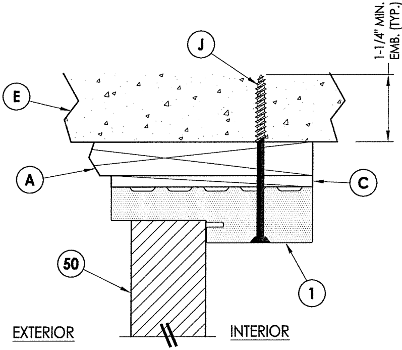
2 6 VERTICAL CROSS SECTION Outswing shown (Inswing similar)
