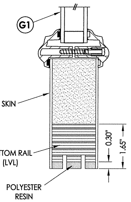
2 2 VERTICAL CROSS SECTION
