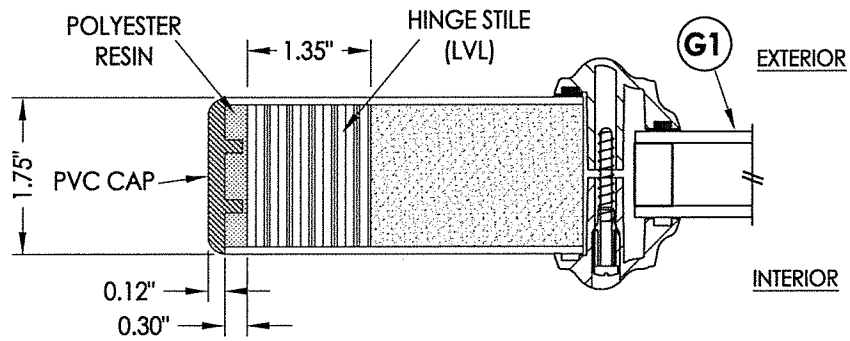
1 HORIZONTAL CROSS SECTION 3
